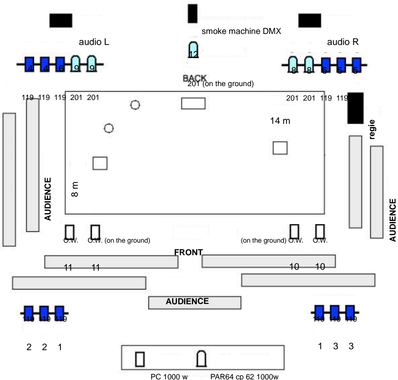
Lichtplan Incontri#2
